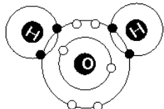
Water molecule
