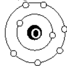
Oxygen atom
