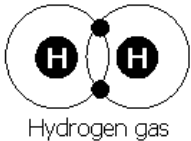
Hydrogen gas
