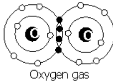
Oxygen gas
